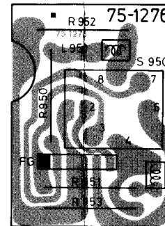
HEADPHONE P.C.B.
