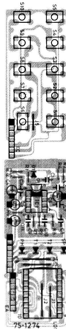
REMOTE CONTROL RECEIVER P.C.B.
